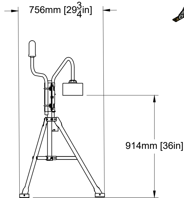
EFM-100 & ANT-2 Sensors on TRI-3 Tripod
